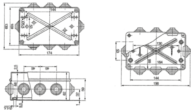
Krabice SolidBOX IP55 / Sealed box IP55 - Obj.č. / Item 68112
