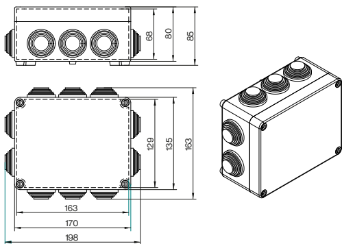
Krabice SolidBOX IP55 / Sealed box IP55 - Obj.č. / Item 68162
