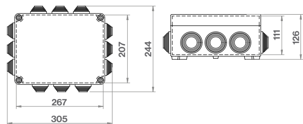
Krabice SolidBOX IP55 / Sealed box IP55 - Obj.č. / Item 68212
