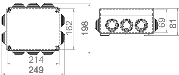
Krabice SolidBOX IP55 / Sealed box IP55 - Obj.č. / Item 68162
