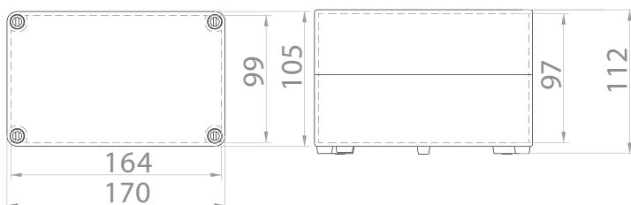
Krabice SolidBOX IP65 / Sealed box IP65 - Obj.č. / Item 68080
