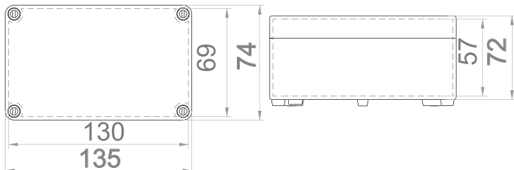
Krabice SolidBOX IP65 / Sealed box IP65 - Obj.č. / Item 68060
