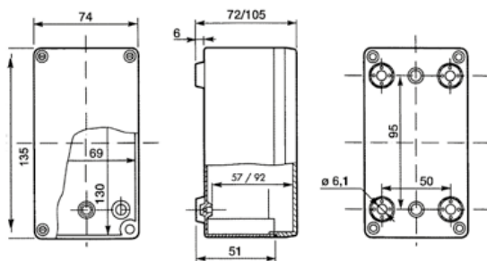
Krabice SolidBOX IP65 / Sealed box IP65 - Obj.č. / Item 68070 / 68071
