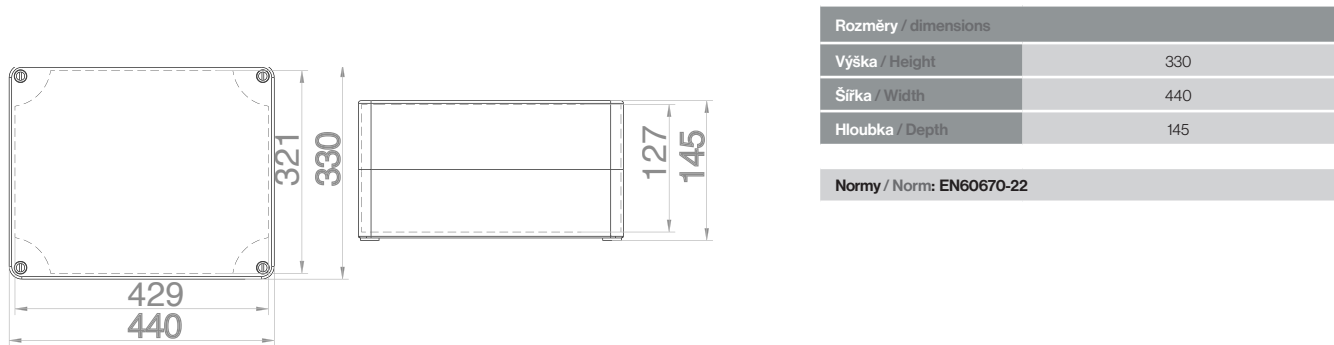
Krabice SolidBOX IP65 / Sealed box IP65 - Obj.č. / Item 68270 / 68271
