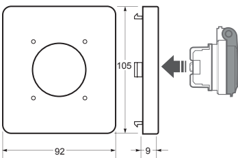
Deska AcquaCOMBI pro zásuvky 50x50 / Socket cover for panel socket 50x50 to mount in Acqua-Combi enclosures
