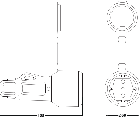
Spojky s gumovou krytkou SCHUKO IP54 / Mobile socket with rubber cover - Obj.č. / Item 2165
