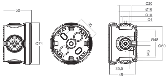
Krabice AcquaBOX IP65 / Box with cones IP65 - Obj.č. / Item 3025
