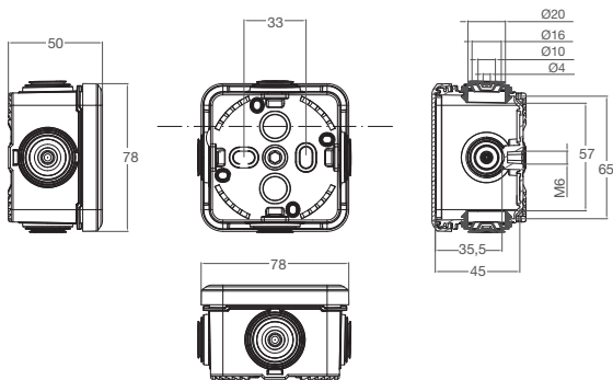
Krabice AcquaBOX IP65 / Box with cones IP65 - Obj.č. / Item 3028
