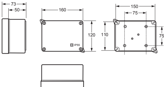
Krabice AcquaBOX IP55 / Sealed box IP55 - Objč. / Item 3042 / 3072
